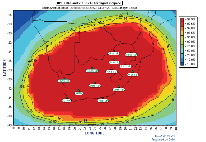
magicSBAS APV-I availability over South Africa
