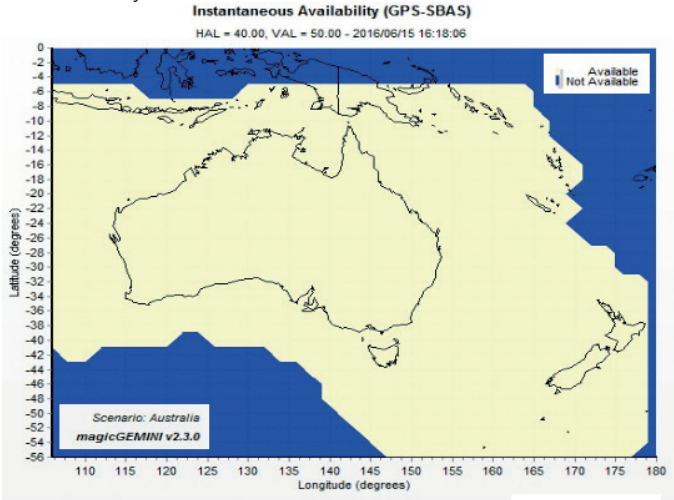
magicSBAS APV-I availability over Australia and New Zealand
